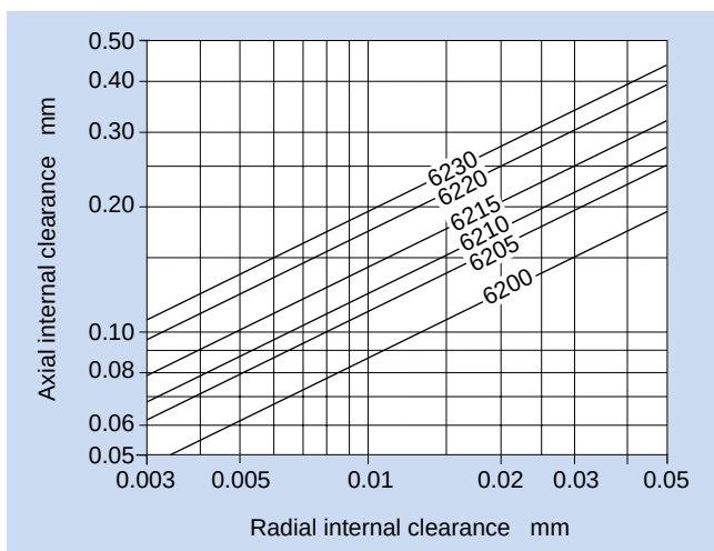
Fig. 17.1.4 Series 62 radial internal/axial internal clearances
