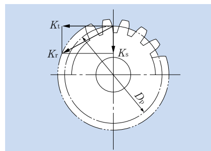
Fig. 4.3 Radial resultant forces
