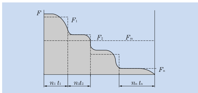
Fig. 4.8 Stepped load
