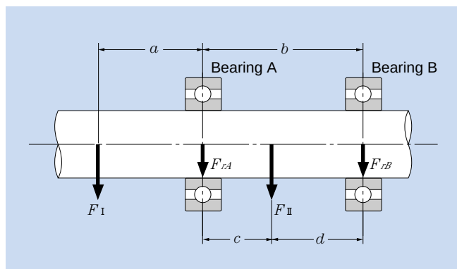
Fig. 4.7 Gear shaft
