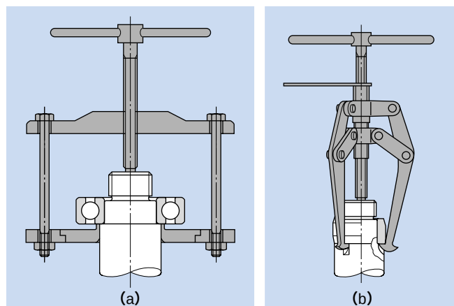
Fig. 15.15 Puller disassembly
