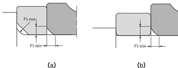
Fig. 14.1 Bearing mounting with spacer
