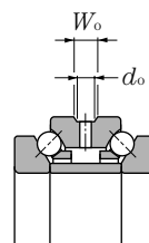
Oil inlet, oil groove dimensions Units mm
