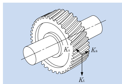
Fig. 4.2 Helical gear loads
