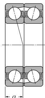
Face-to-face arrangement (DF)
