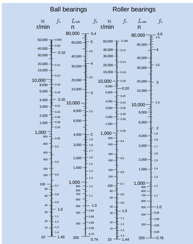
Fig. 3.1 Bearing life rating scale
