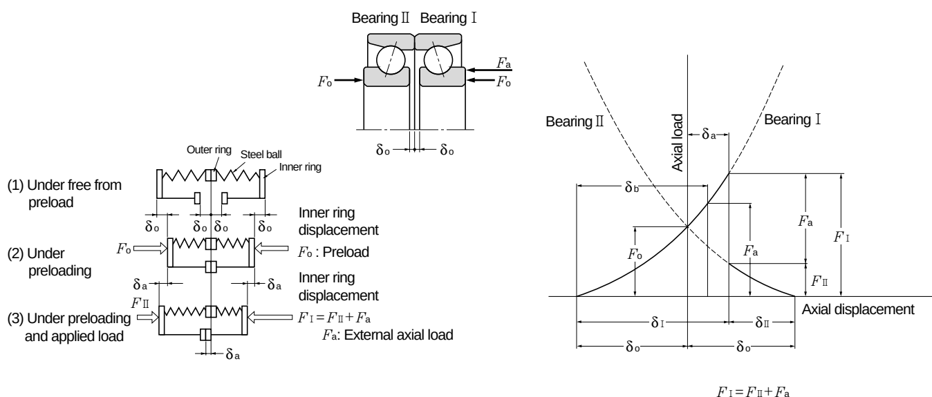
Fig. 8.2 Fixed position preload versus axial displacement
