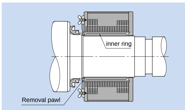
Fig. 15.6 Removal of inner ring using an induction heater
