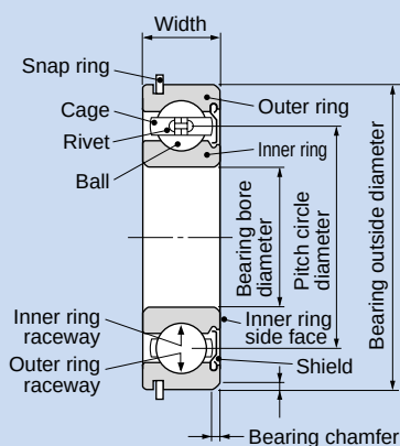
Deep groove ball bearing
