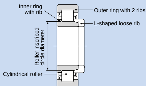
Cylindrical roller bearing
