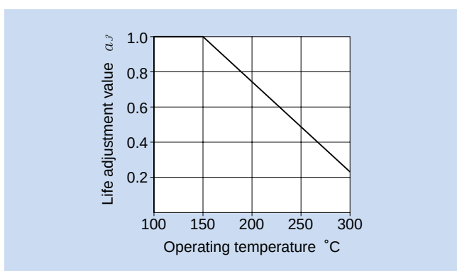
Fig. 3.2 Life adjustment value for operating temperature
