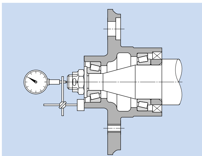
Fig. 15.13 Measurement of axial internal clearance adjustment
