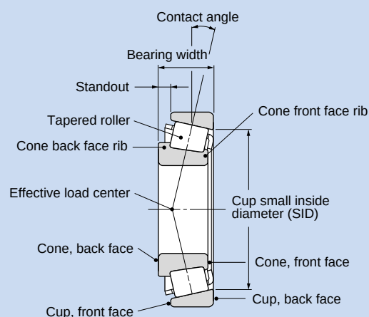
Tapered roller bearing
