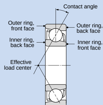
Angular contact ball bearing
