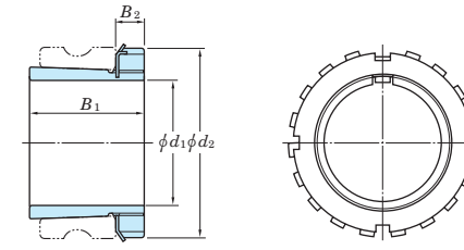
Adapter assembly
