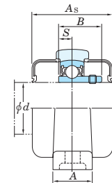
Open ends type
