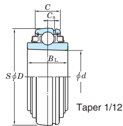
UK...L3 (with triple-lip seals)
