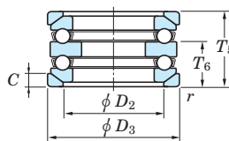
With aligning seat races
