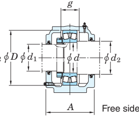
SSN 2, 3 Different bore type (locknut locking)
