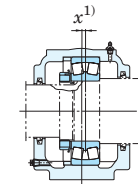
Fixed side (When one stabilizing ring used)
