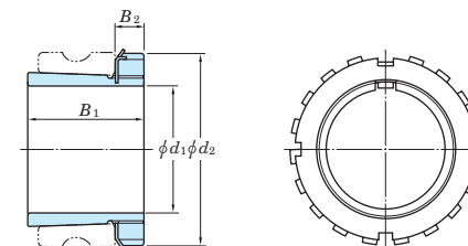
Adapter assembly
