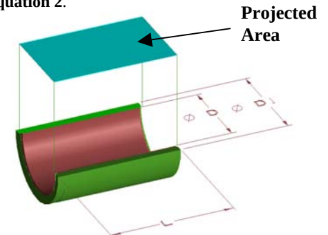
Figure 4, (Non-flanged Journal)
