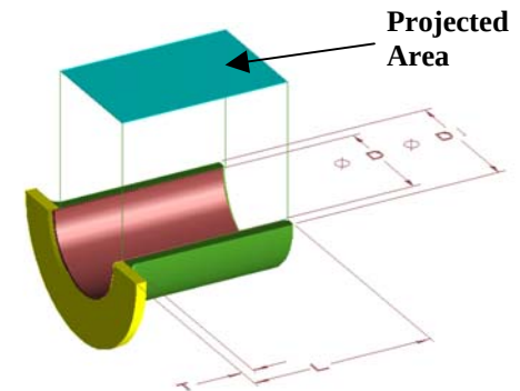
Figure 4, (Flanged Journal)
