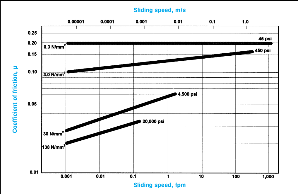
Figure 4-2. Friction vs. Velocity for Various Loads
