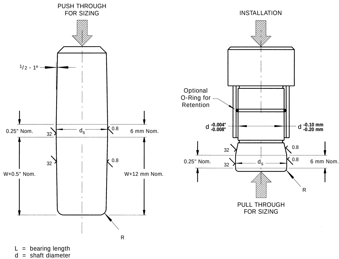
Figure 6-3. Burnishing Tools
