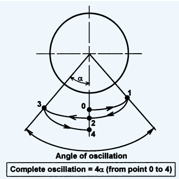
Figure 5-2. Oscillation Angle
