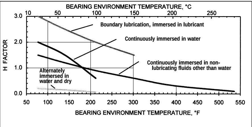
Figure 4-7. DU Heat Dissipation Factor – H for Fluid Applications
